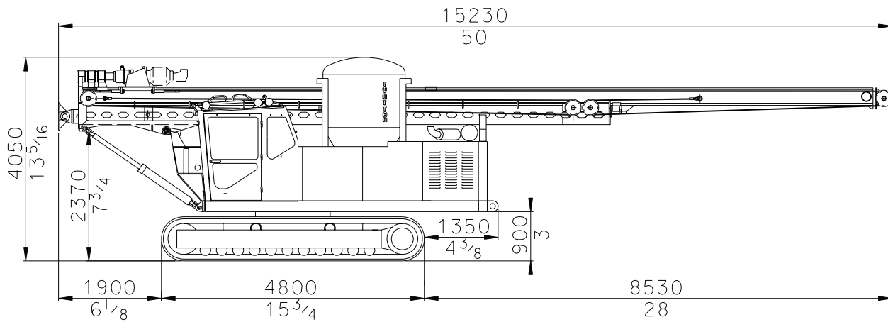
DS15 transport dimensions.
