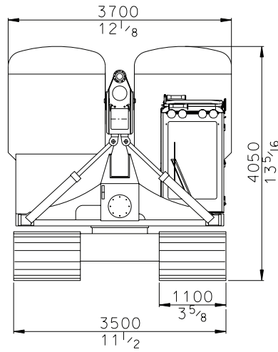
Width and height.
